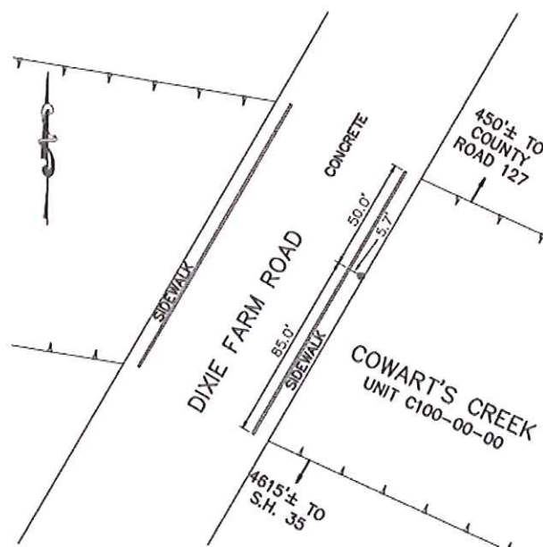
Detail Sketch
